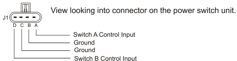
Connector Pin Layout:
