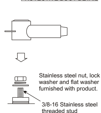
PROTECTIVE BOOT DETAIL
