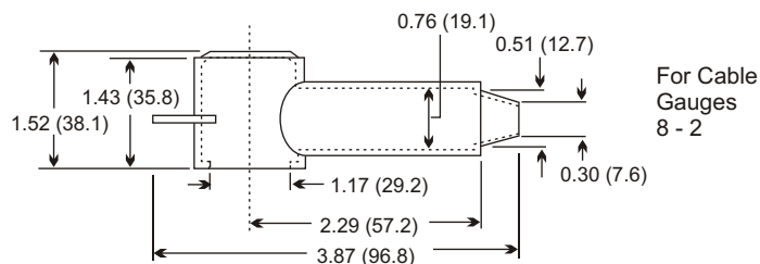
Rubber Boot Detail
